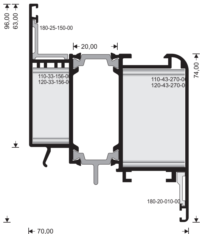
KRILO VELIKO-RAVNO SASH LARGE FLAT
